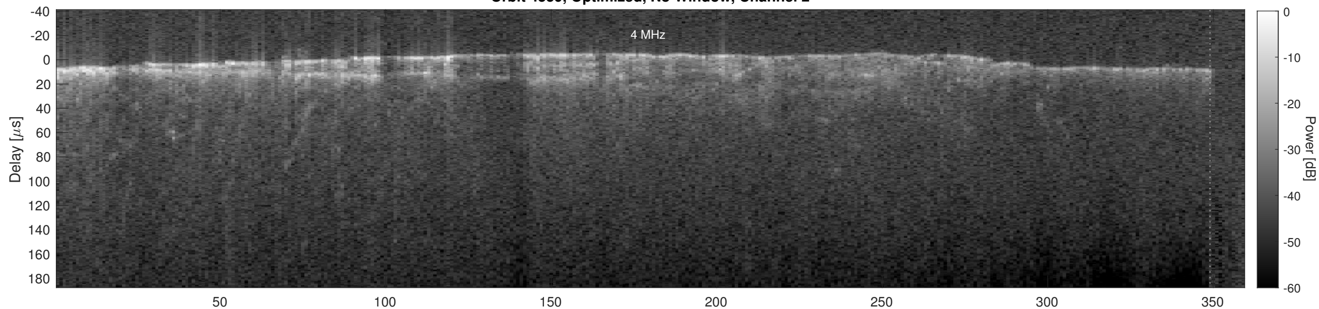
Orbit 4559, Cluttergram
