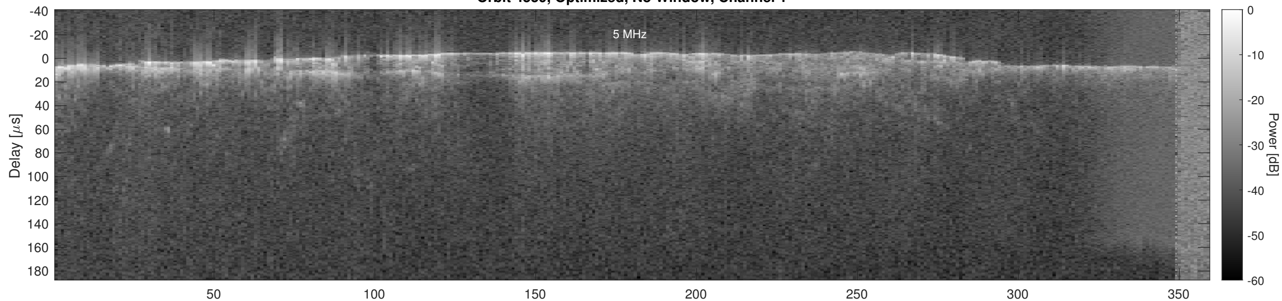
Orbit 4559, Optimized, No Window, Channel 2
