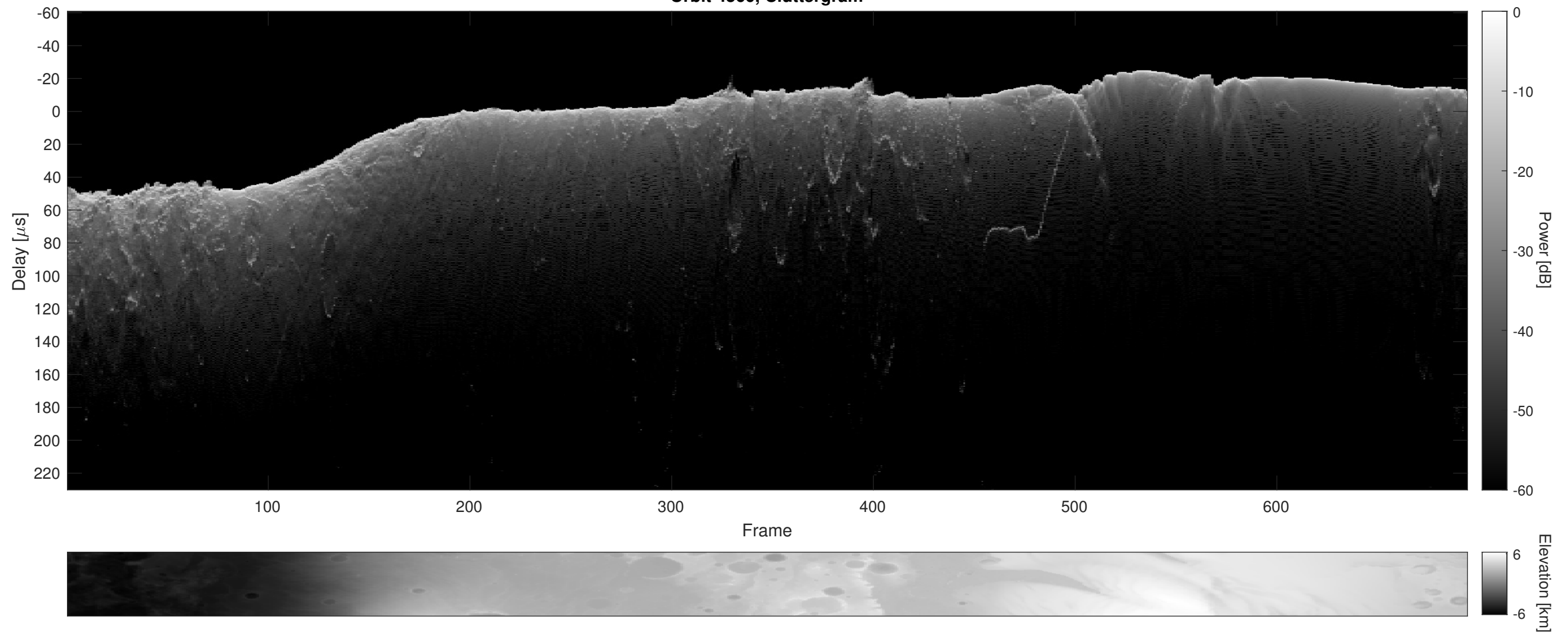
Orbit 4560, Cluttergram
