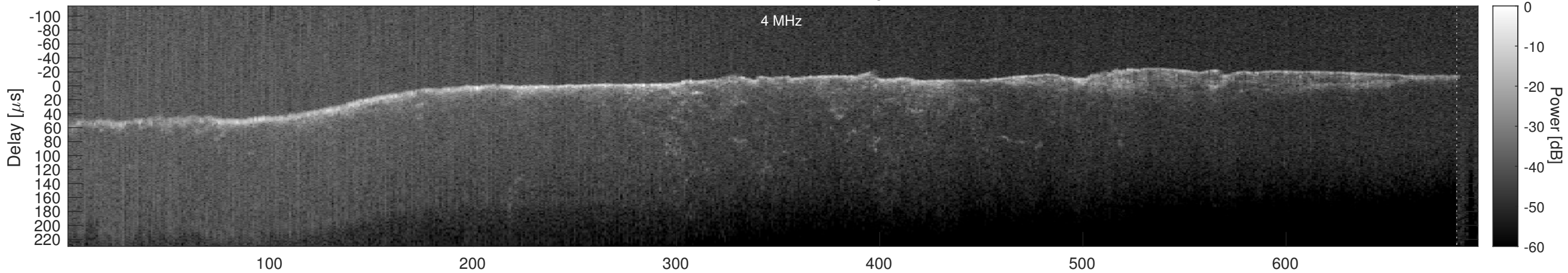
Orbit 4560, Cluttergram
