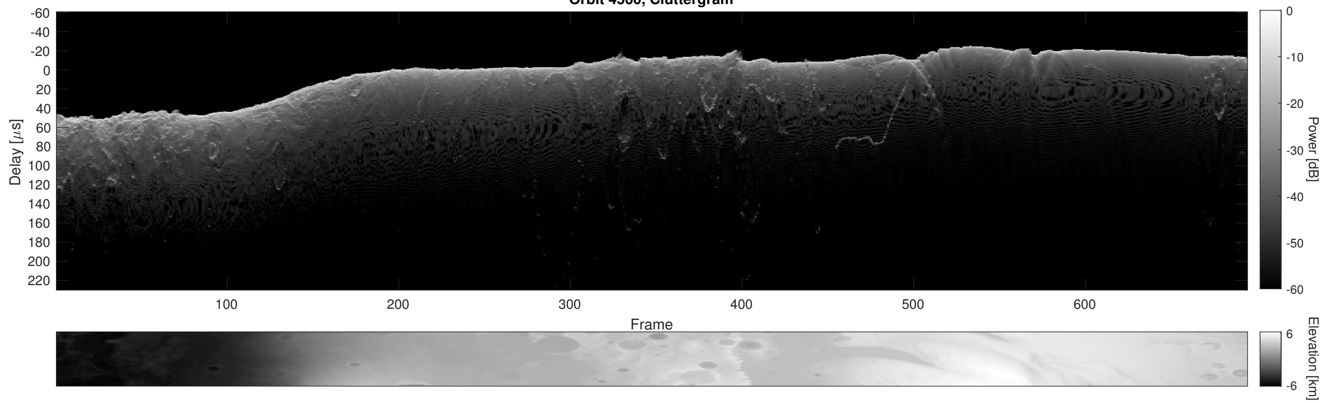
Orbit 4560, Cluttergram
