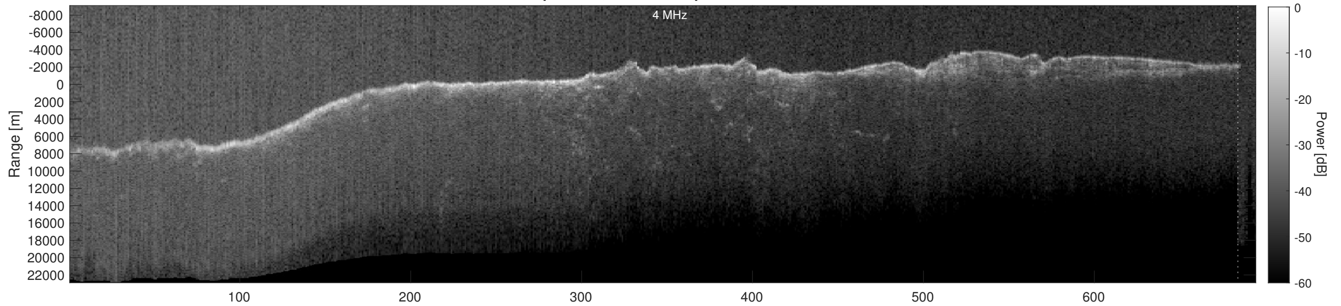
Orbit 4560, Depth-Corrected Cluttergram
