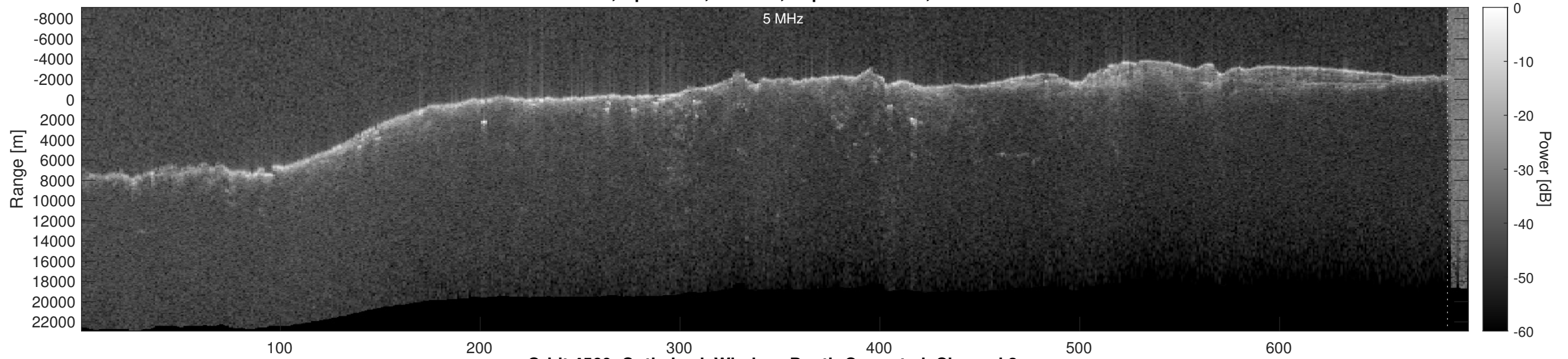
Orbit 4560, Optimized, Window, Depth-Corrected, Channel 2
