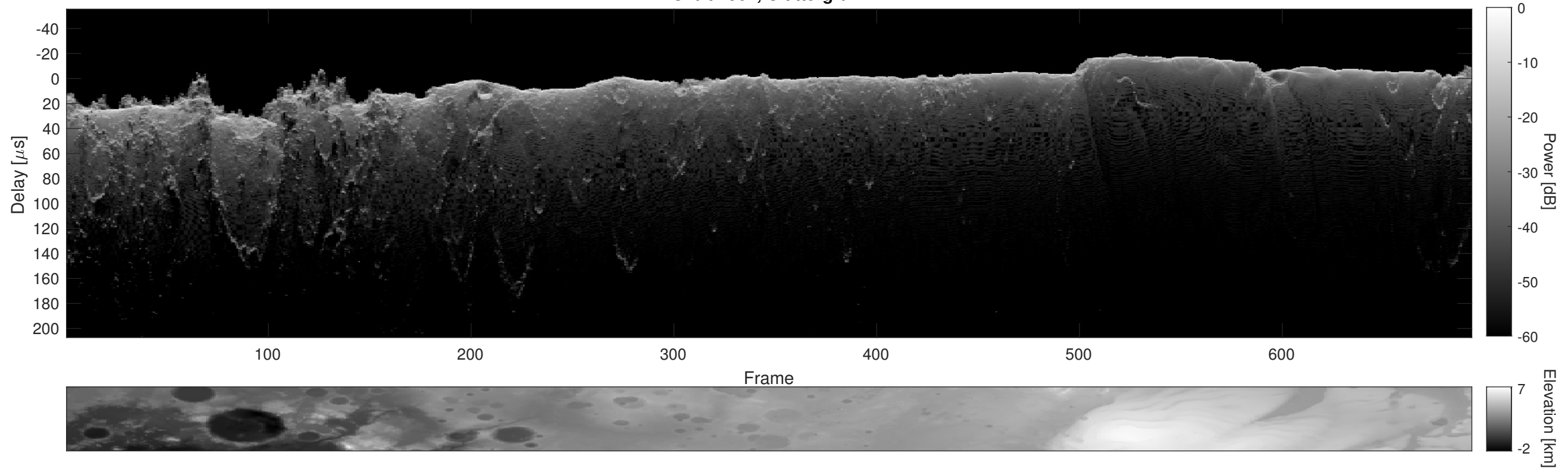
Orbit 4561, Cluttergram
