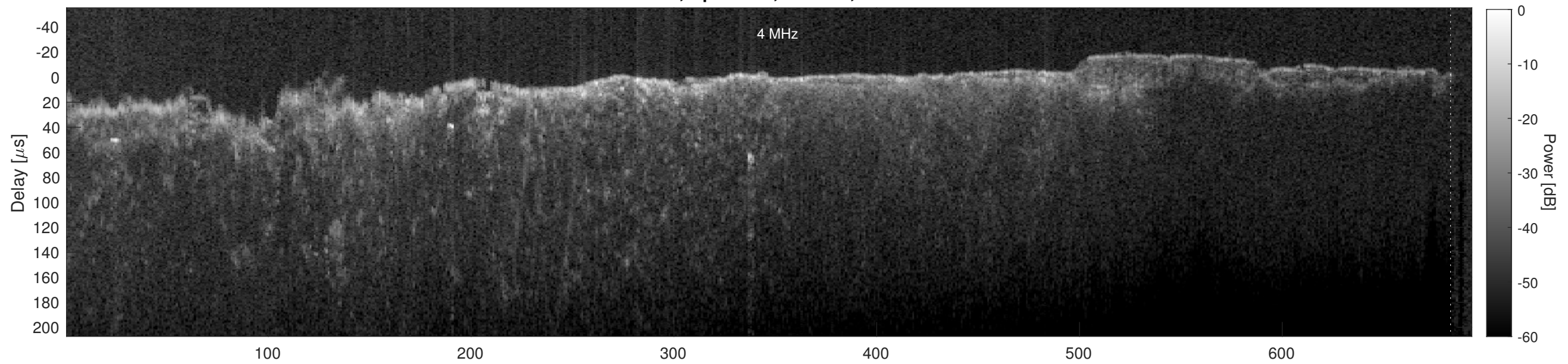
Orbit 4561, Cluttergram
