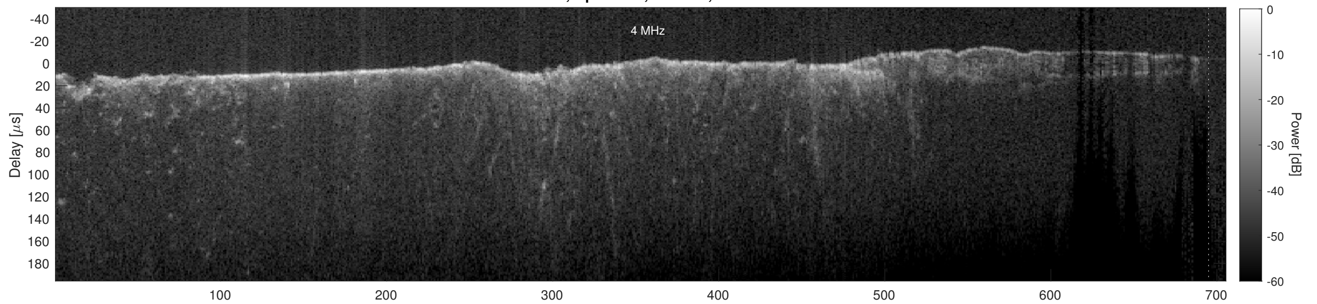
Orbit 4564, Cluttergram
