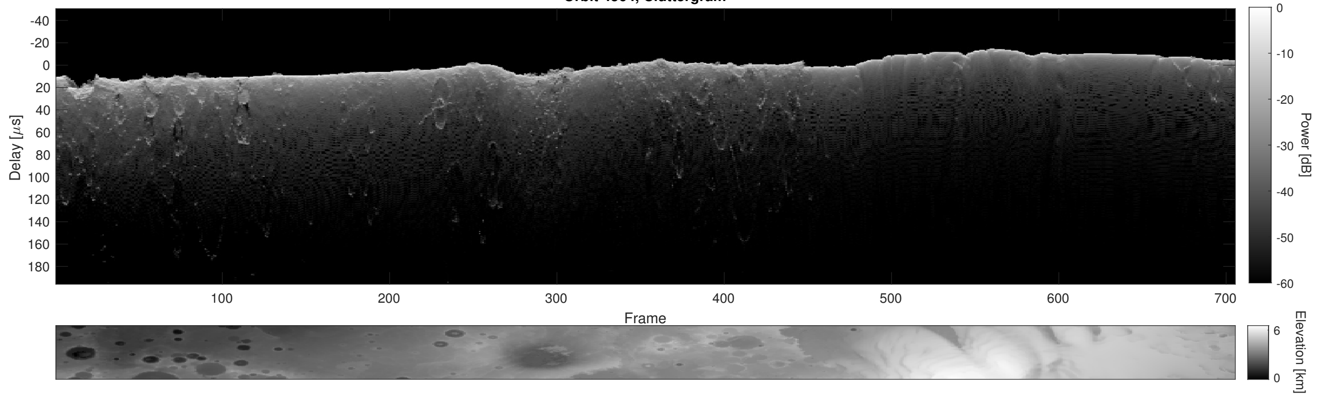
Orbit 4564, Cluttergram
