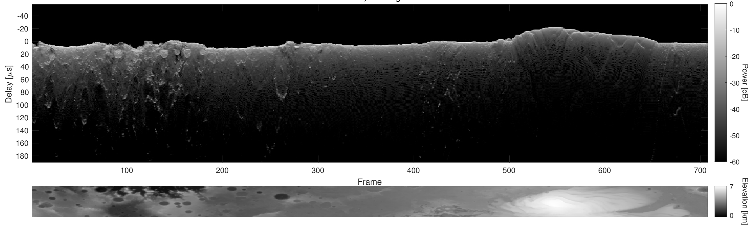
Orbit 4565, Cluttergram
