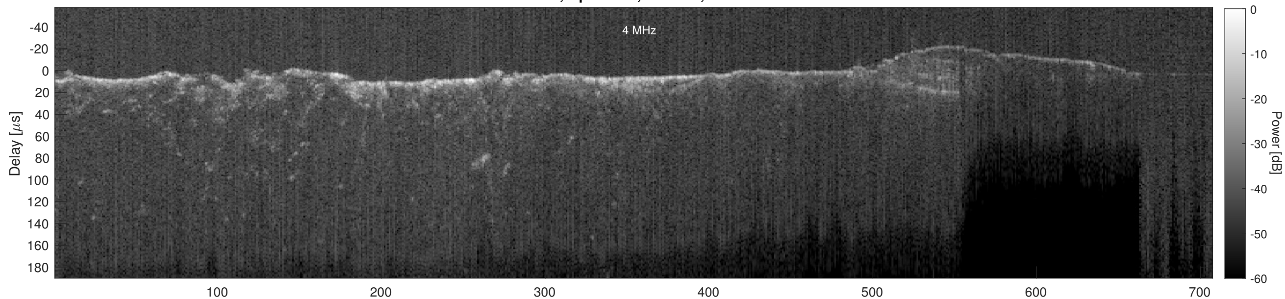
Orbit 4565, Cluttergram
