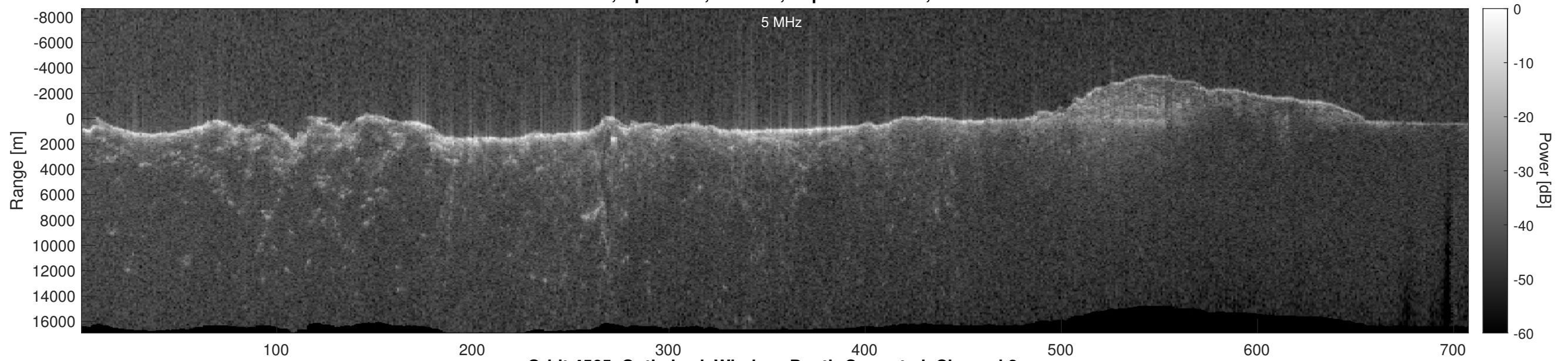
Orbit 4565, Optimized, Window, Depth-Corrected, Channel 2
