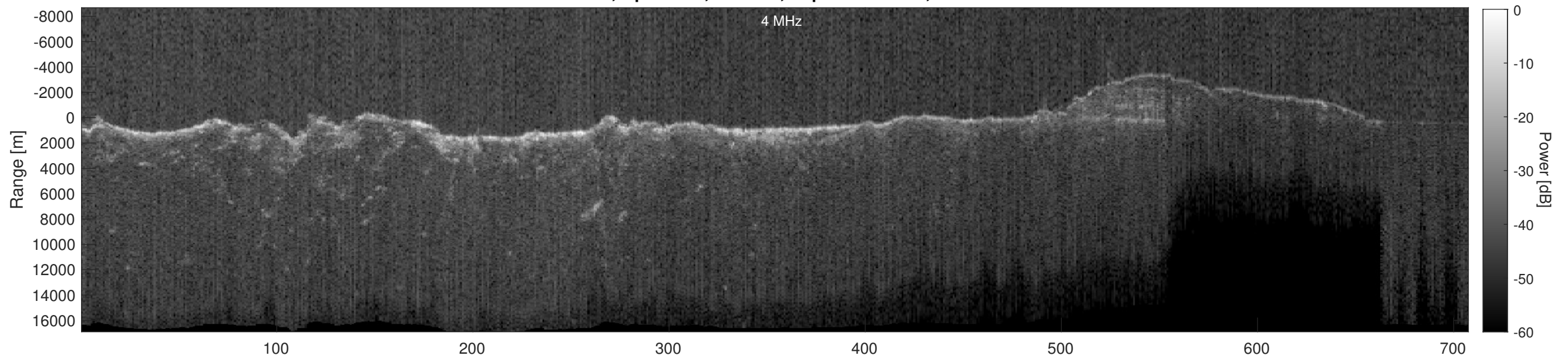
Orbit 4565, Depth-Corrected Cluttergram
