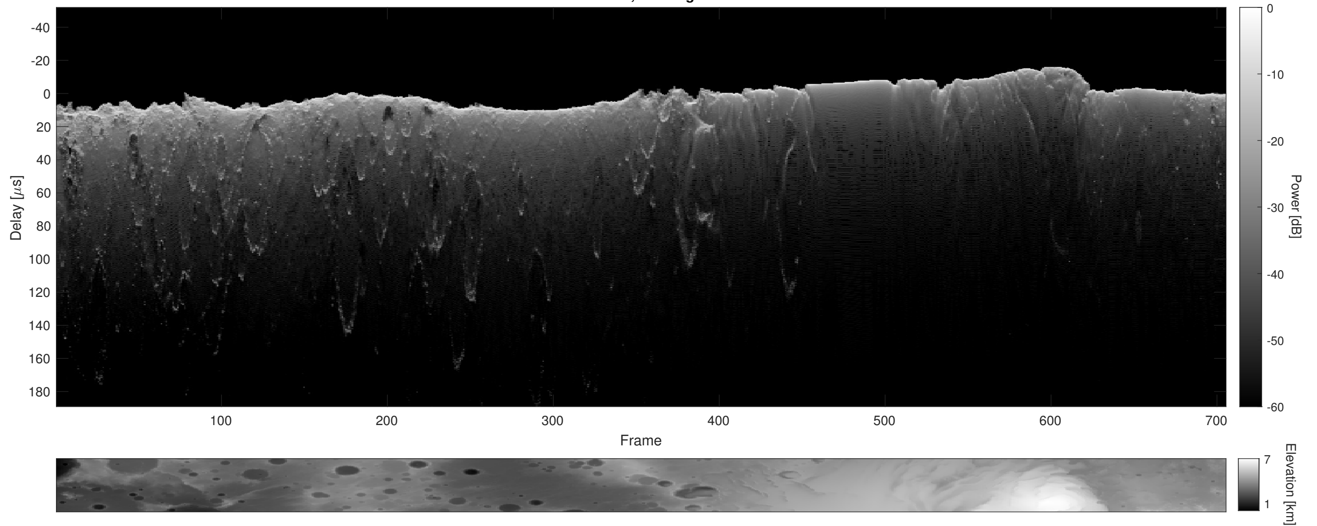
Orbit 4566, Cluttergram
