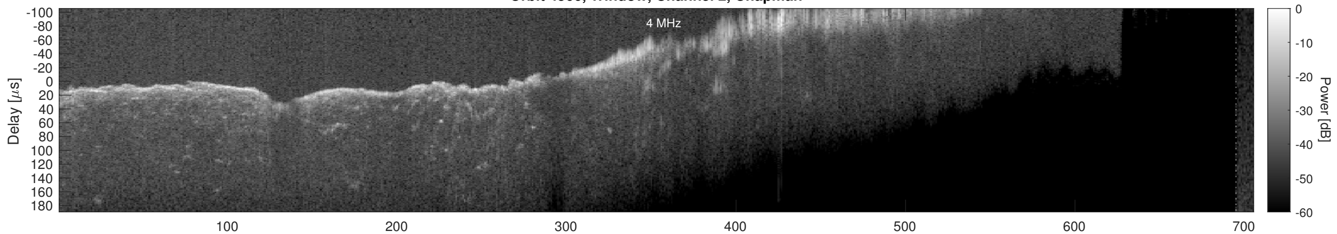
Orbit 4566, Window, Channel 2, Optimized
