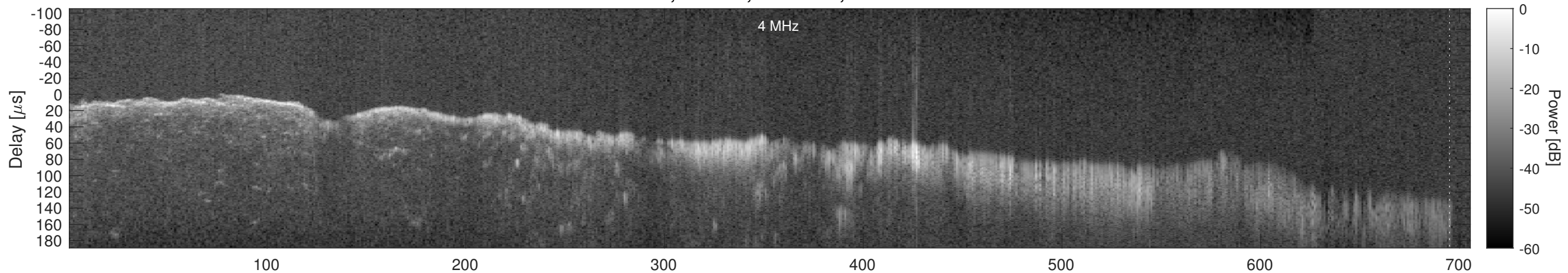
Orbit 4566, Window, Channel 2, Chapman
