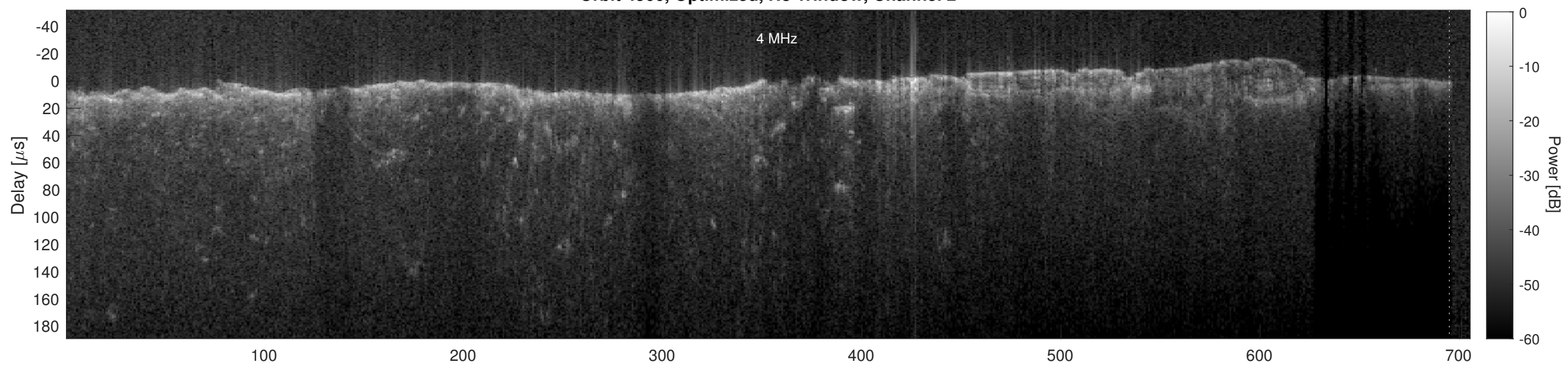
Orbit 4566, Cluttergram
