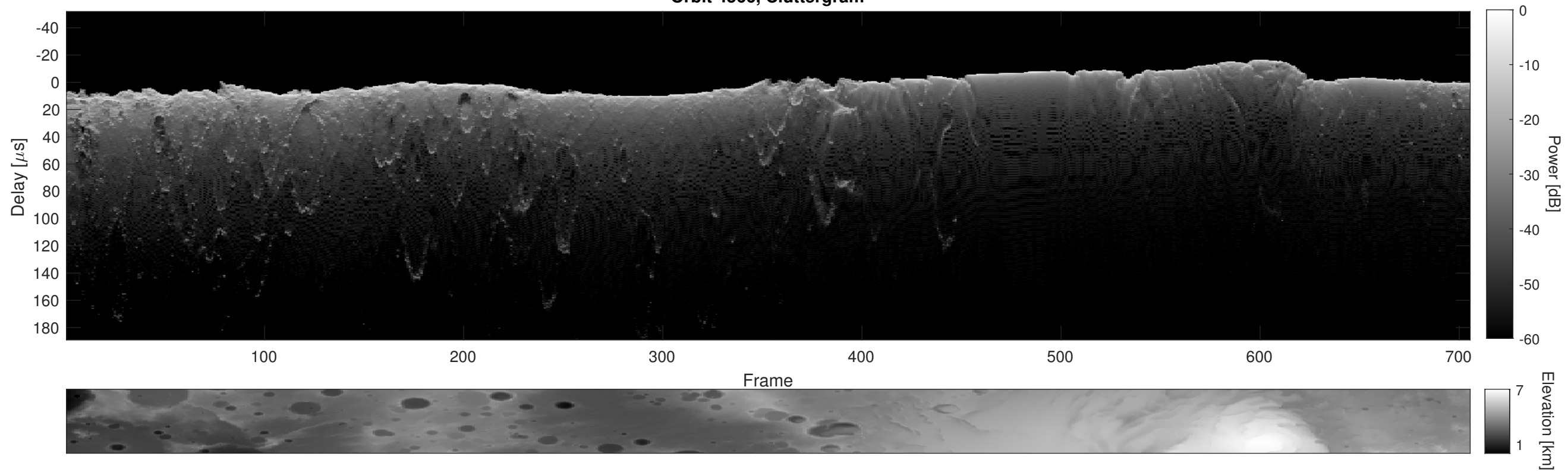
Orbit 4566, Cluttergram
