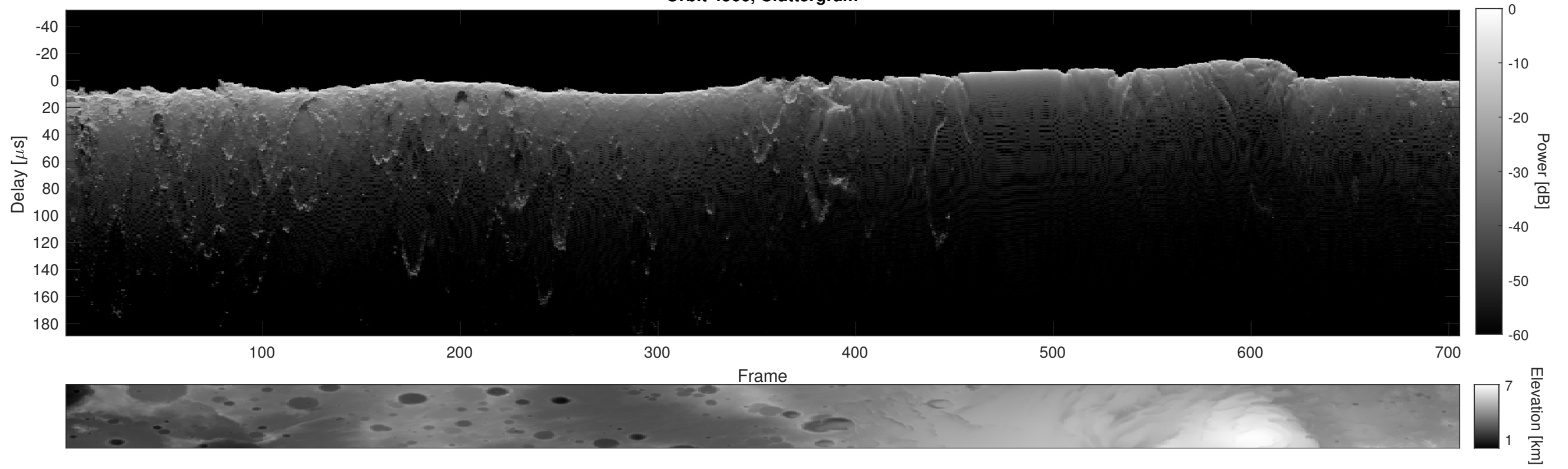
Orbit 4566, Cluttergram
