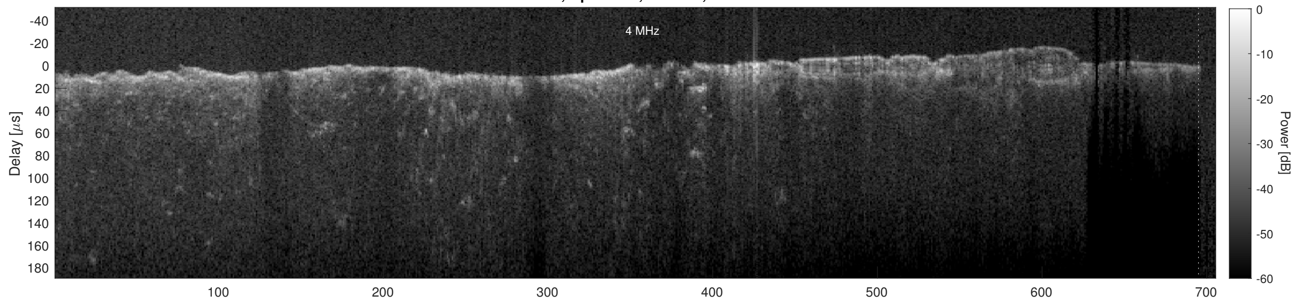
Orbit 4566, Cluttergram
