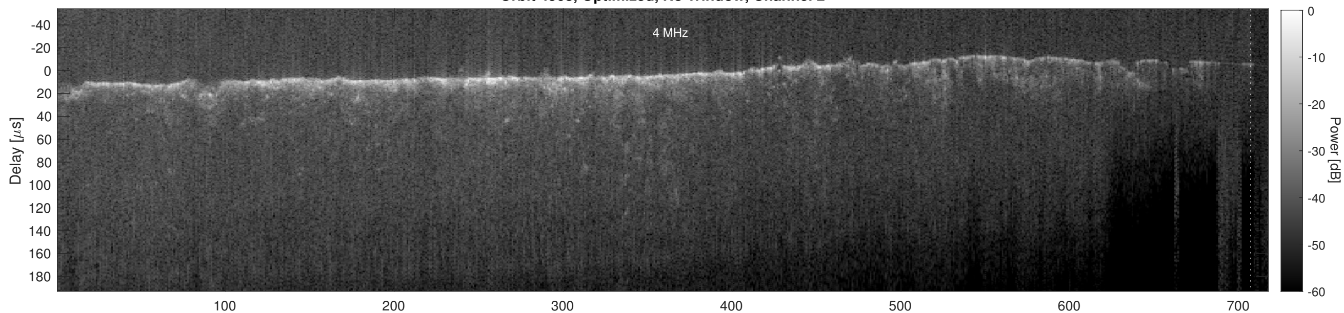
Orbit 4568, Cluttergram
