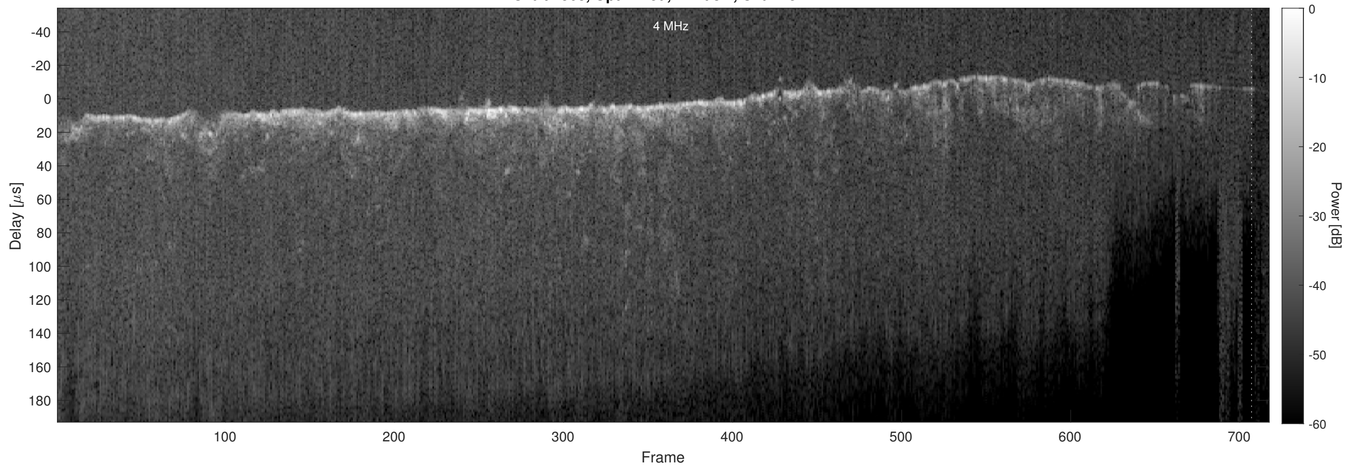
Orbit 4568, Optimized, Window, Channel 2
