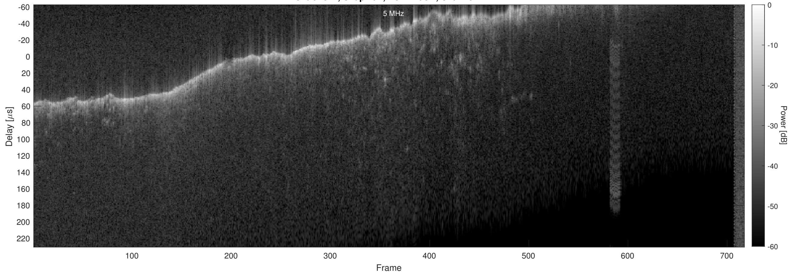
Orbit 4571, Chapman, No Window, Channel 2
