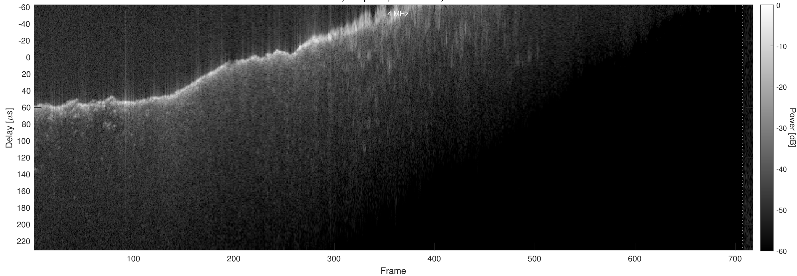
Orbit 4571, Chapman, No Window, Channel 2
