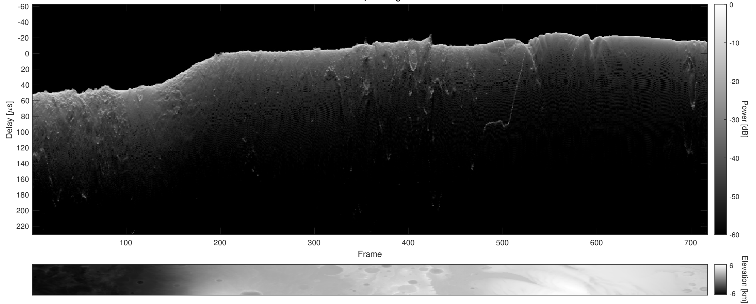
Orbit 4571, Cluttergram
