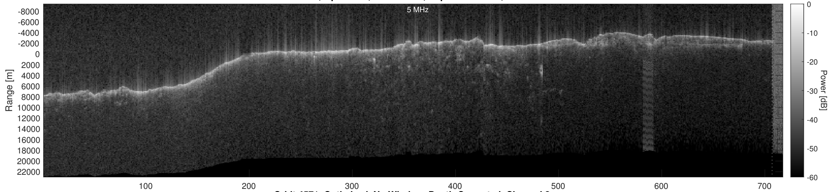
Orbit 4571, Optimized, No Window, Depth-Corrected, Channel 2
