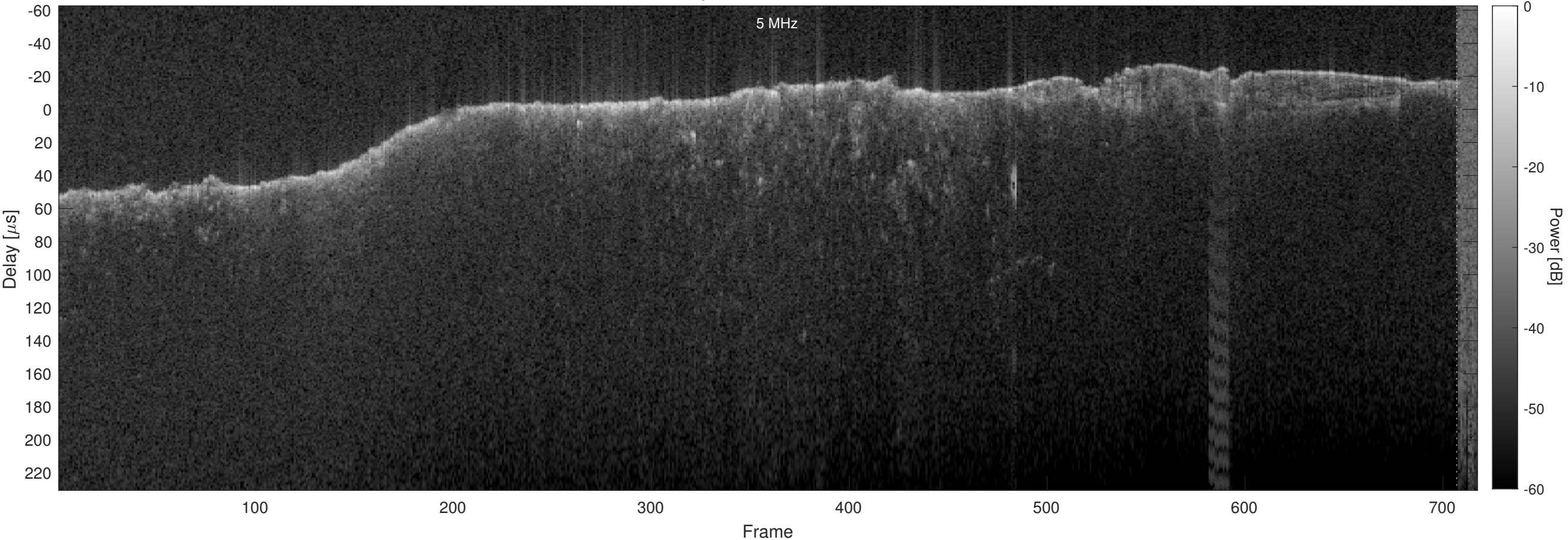
Orbit 4571, Optimized, Window, Channel 2
