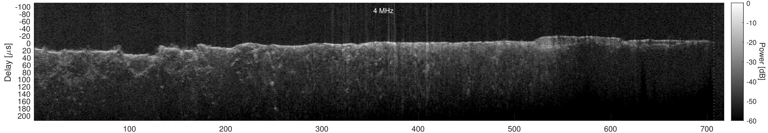
Orbit 4572, Cluttergram
