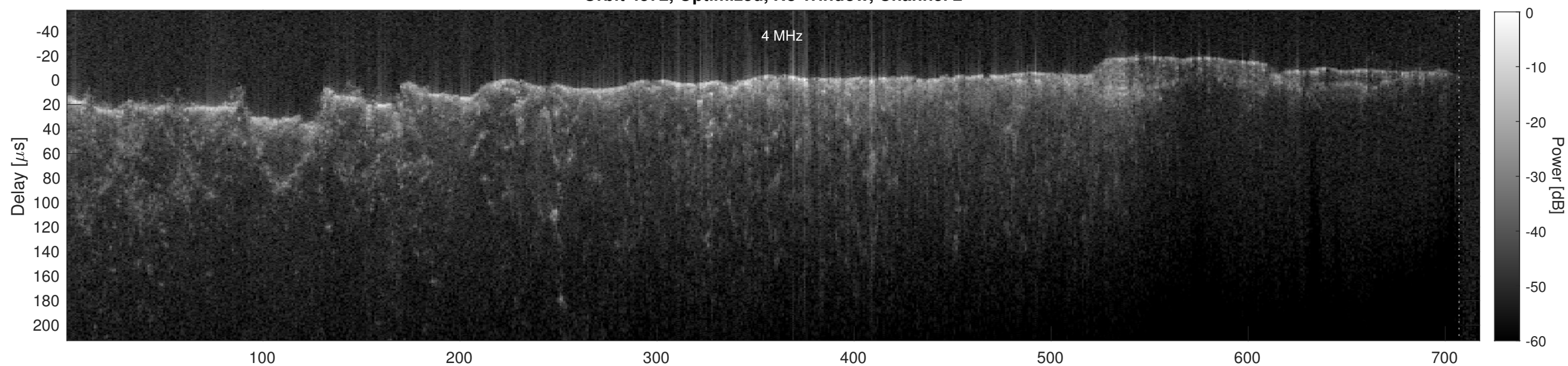
Orbit 4572, Cluttergram
