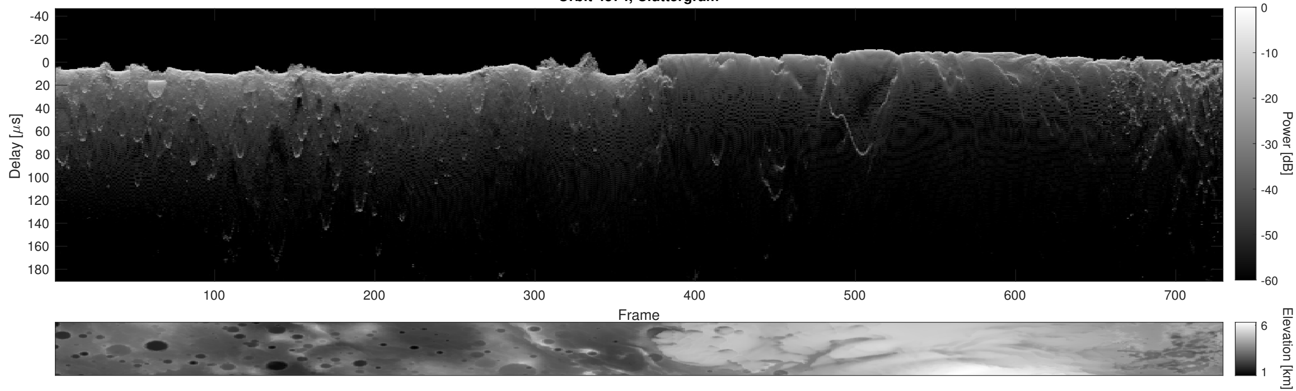
Orbit 4574, Cluttergram
