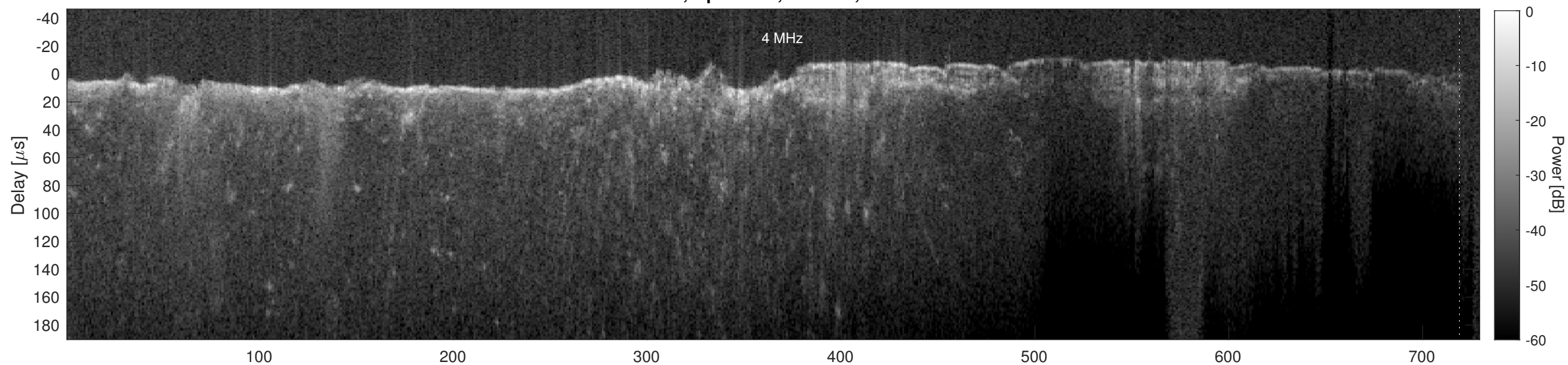
Orbit 4574, Cluttergram
