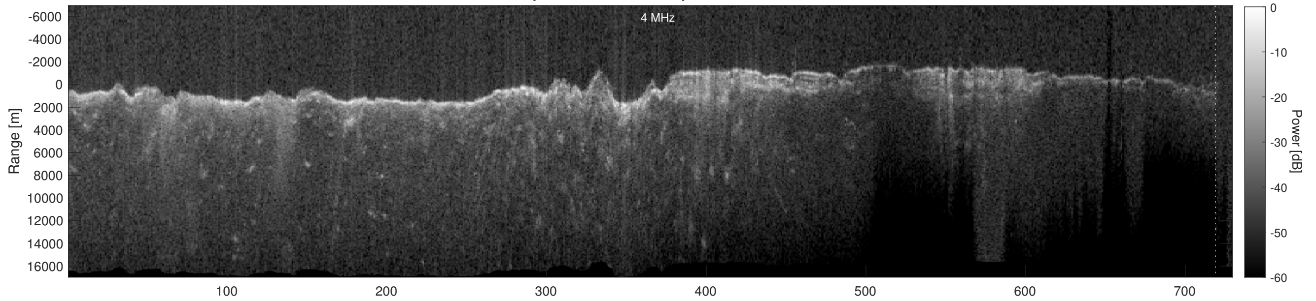
Orbit 4574, Depth-Corrected Cluttergram
