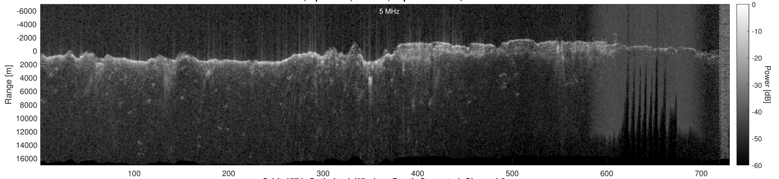
Orbit 4574, Optimized, Window, Depth-Corrected, Channel 2
