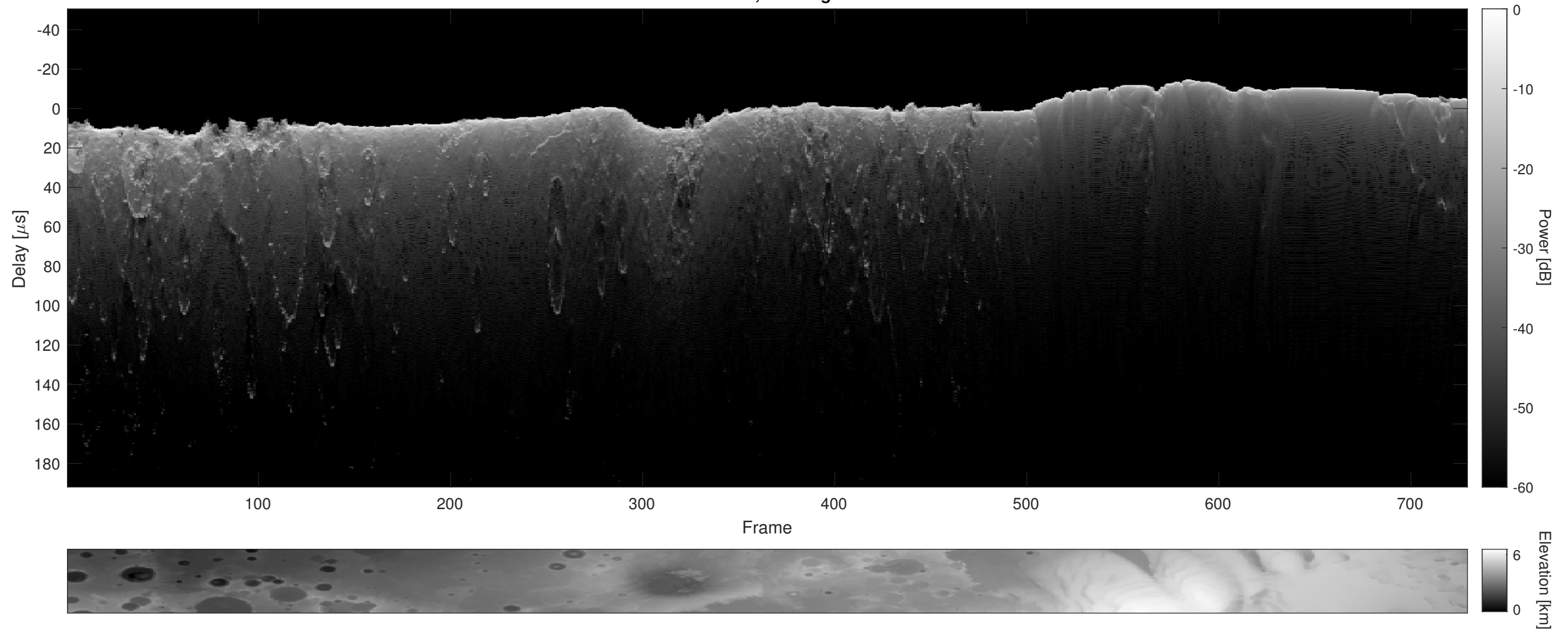
Orbit 4575, Cluttergram
