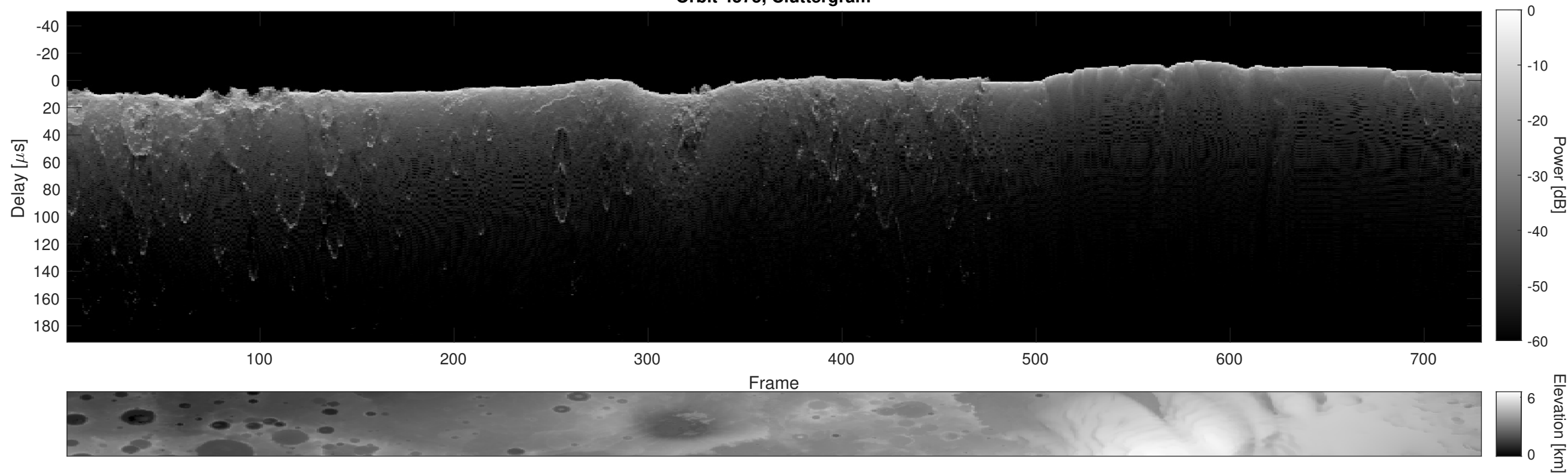
Orbit 4575, Cluttergram
