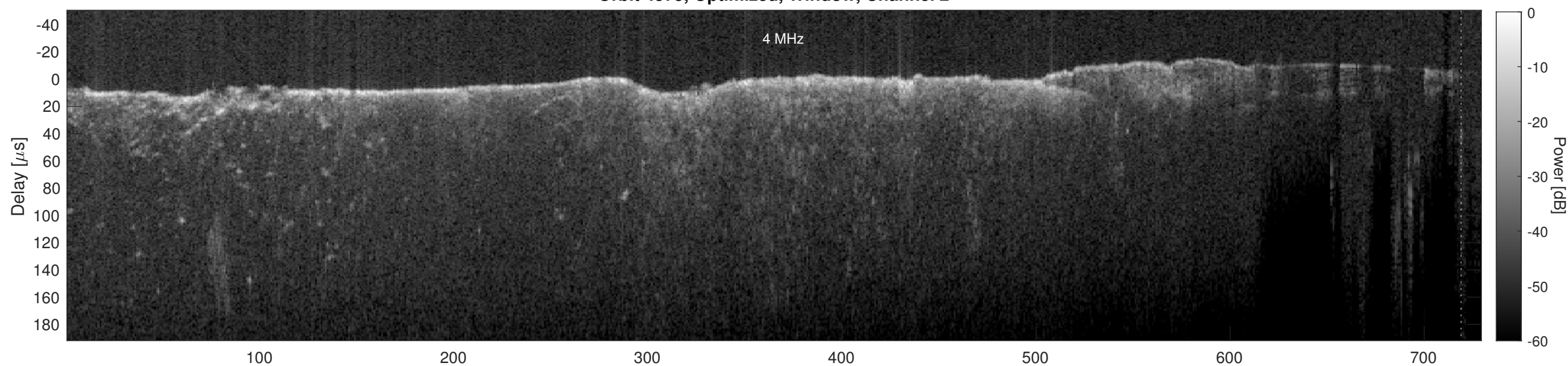
Orbit 4575, Cluttergram
