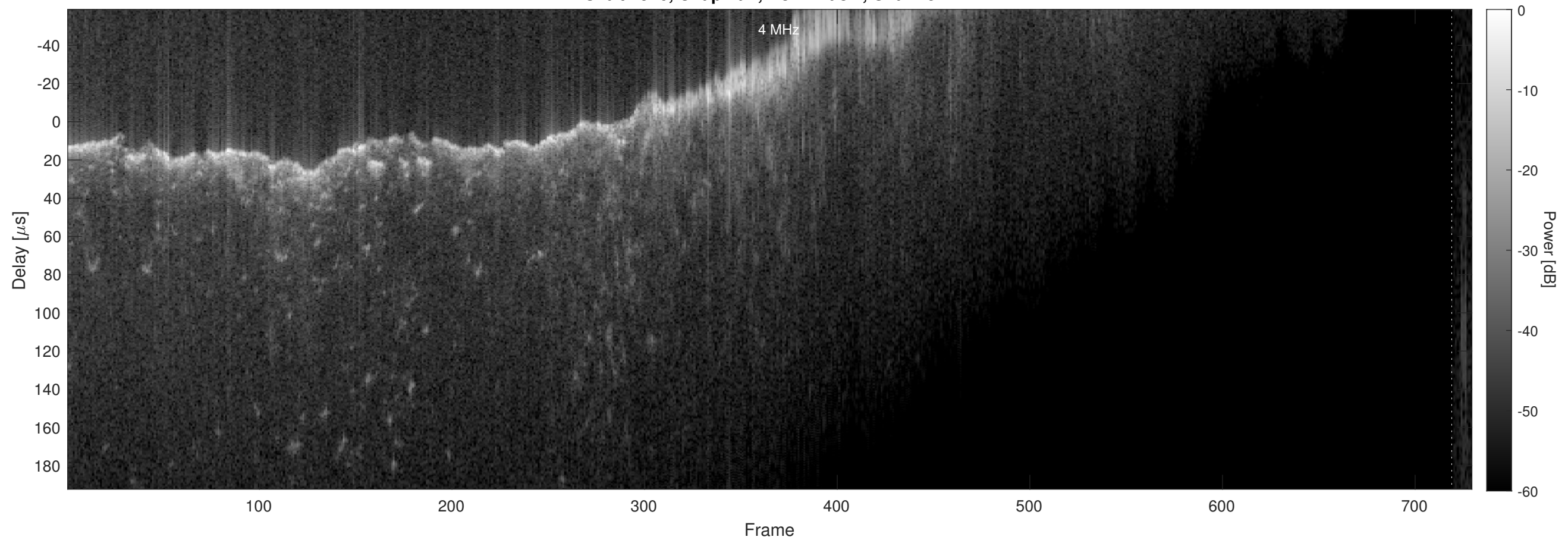
Orbit 4576, Chapman, No Window, Channel 2
