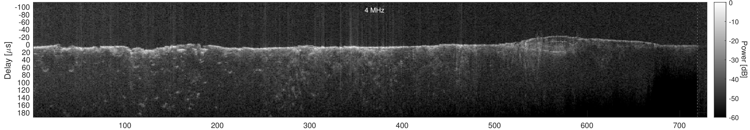
Orbit 4576, Cluttergram
