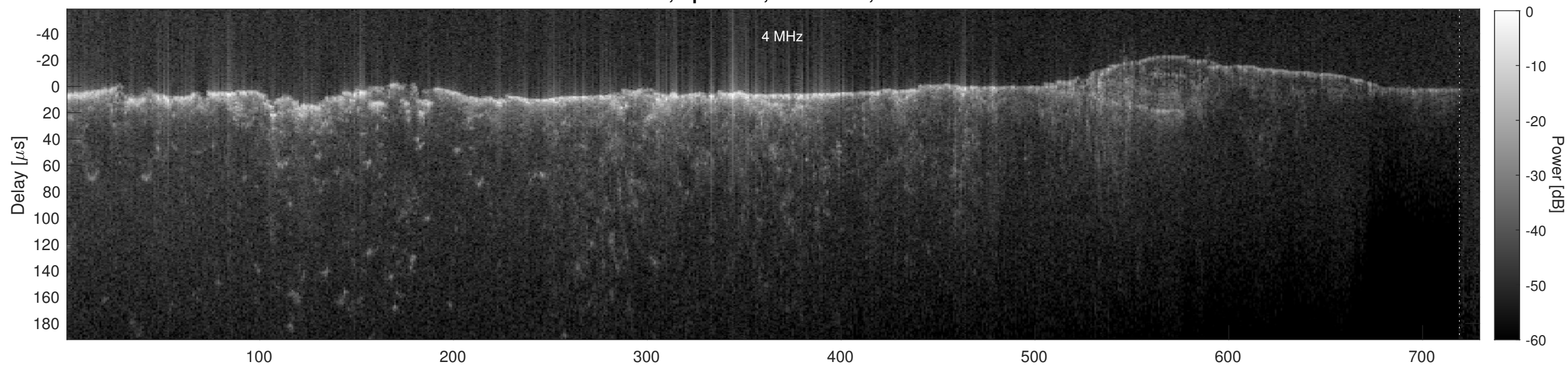
Orbit 4576, Cluttergram
