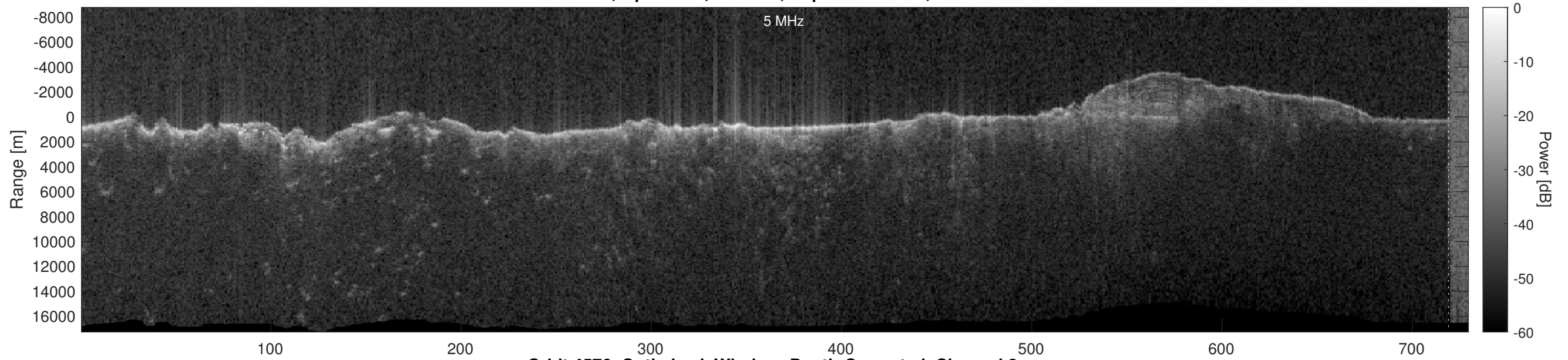
Orbit 4576, Optimized, Window, Depth-Corrected, Channel 2
