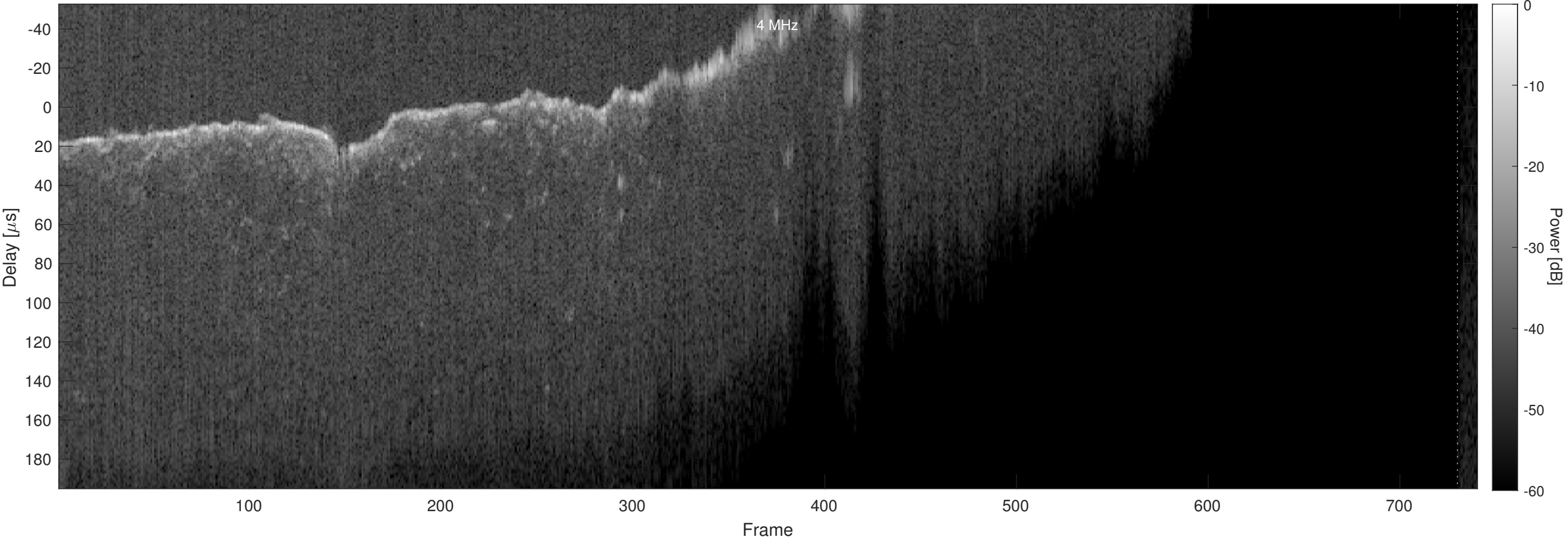
Orbit 4577, Chapman, Window, Channel 2
