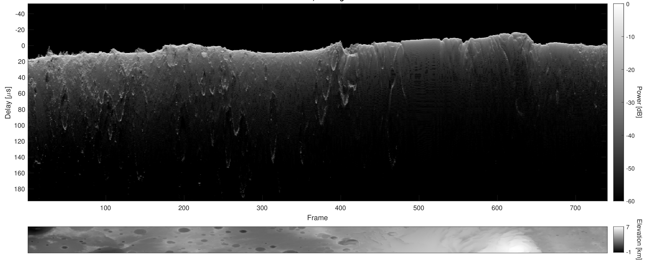
Orbit 4577, Cluttergram
