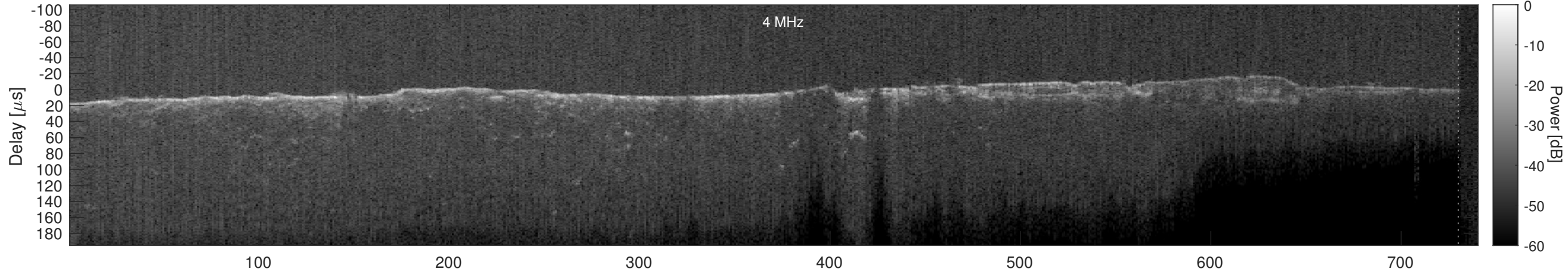
Orbit 4577, Cluttergram
