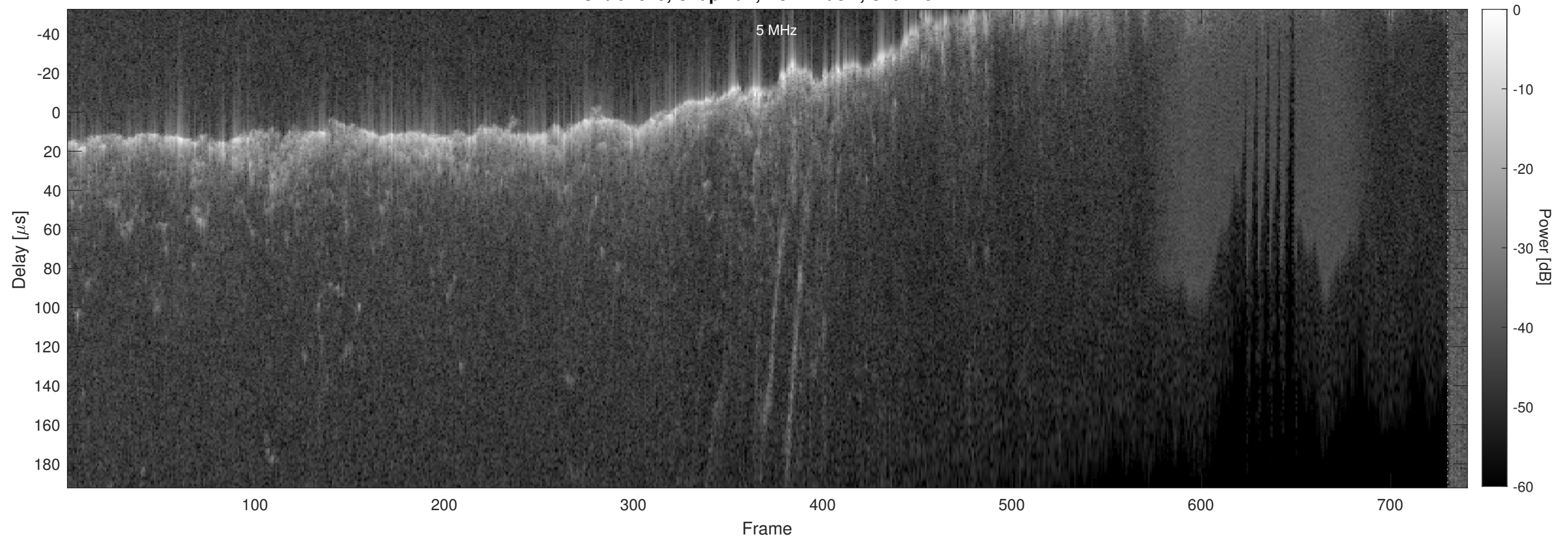
Orbit 4579, Chapman, No Window, Channel 2
