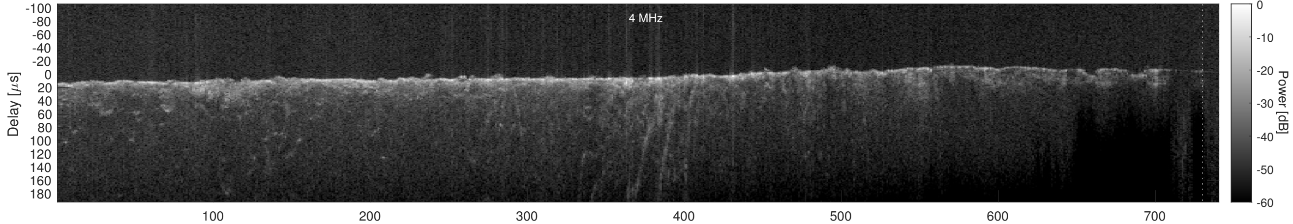
Orbit 4579, Cluttergram
