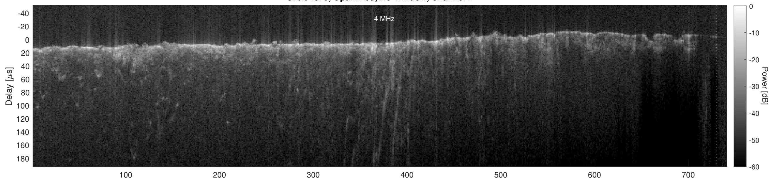
Orbit 4579, Cluttergram
