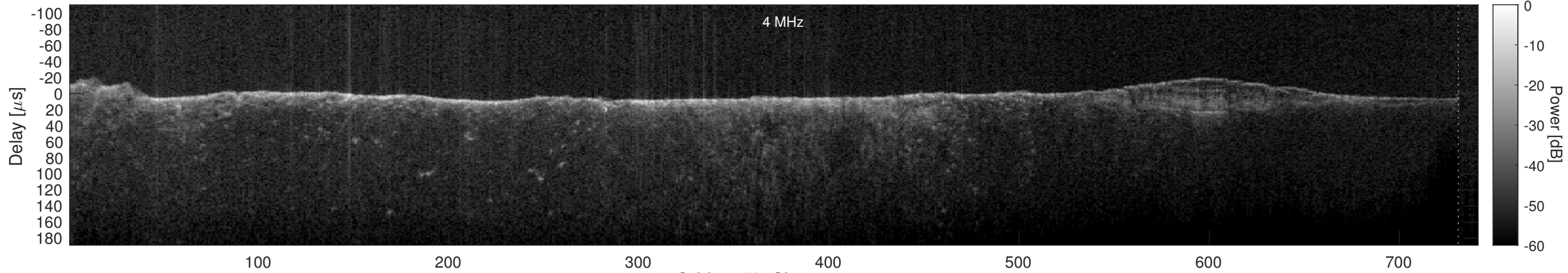
Orbit 4580, Cluttergram
