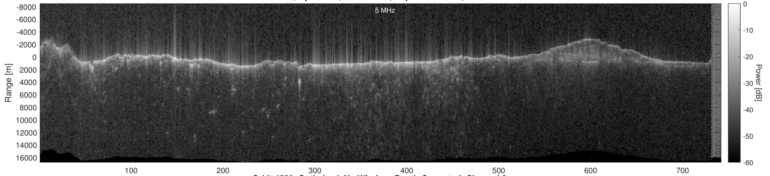
Orbit 4580, Optimized, No Window, Depth-Corrected, Channel 2
