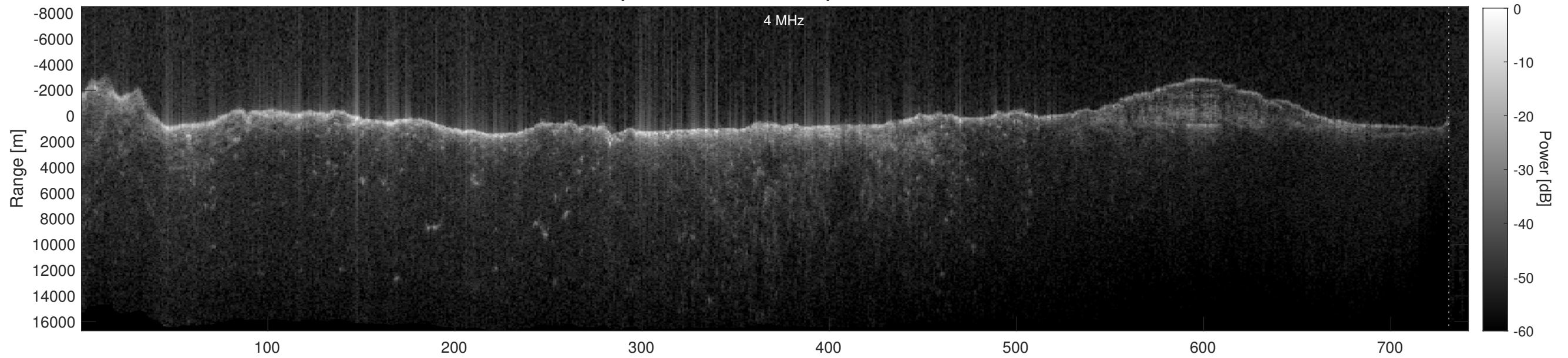
Orbit 4580, Depth-Corrected Cluttergram
