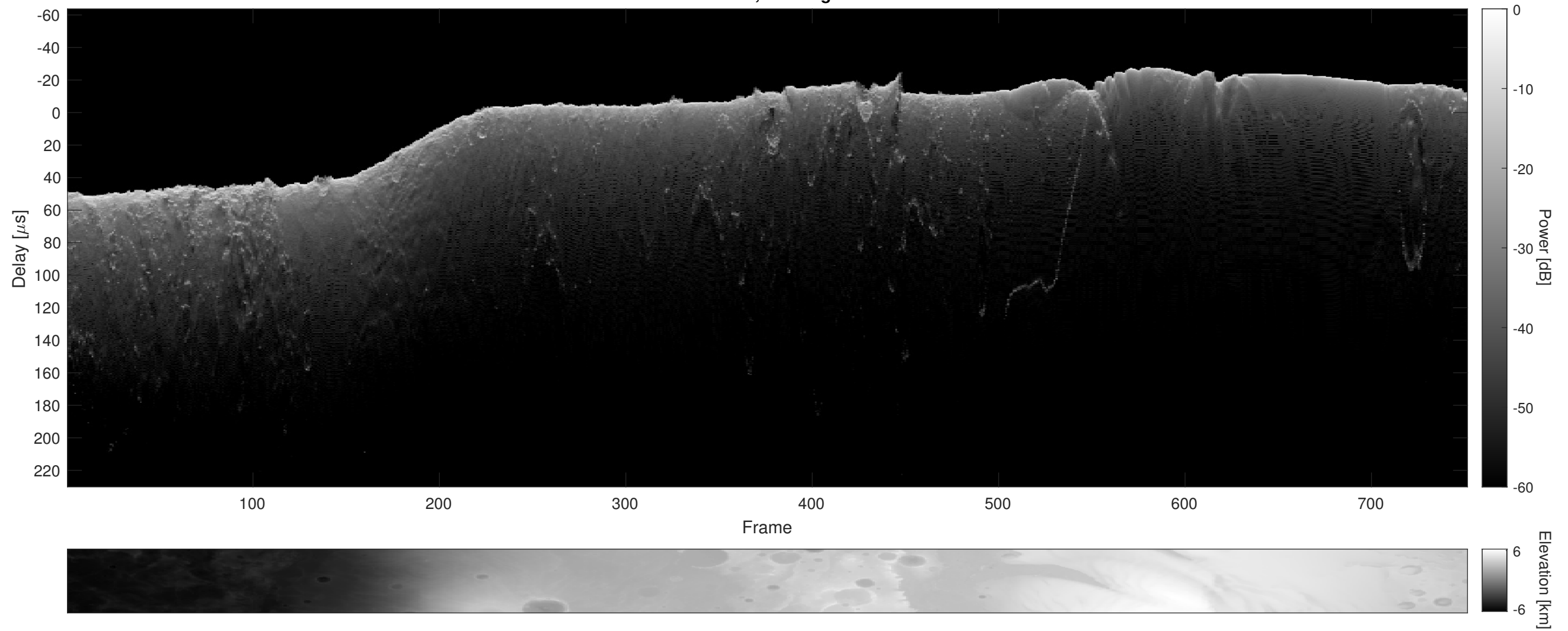
Orbit 4582, Cluttergram
