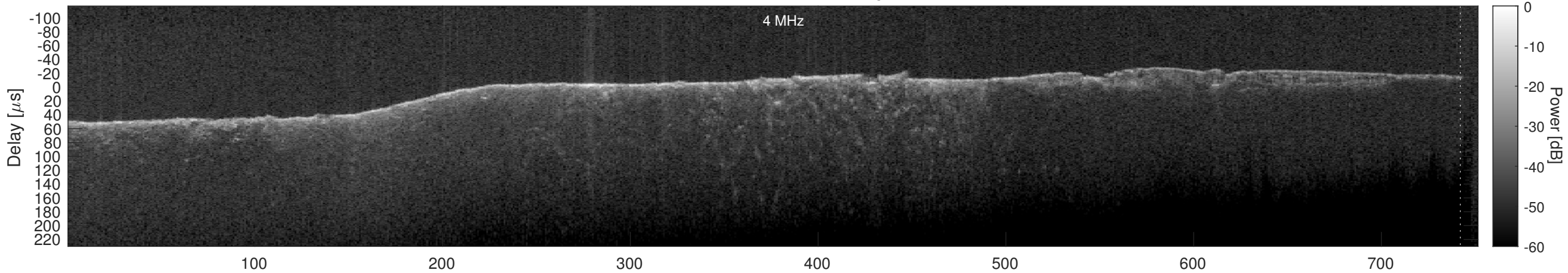
Orbit 4582, Cluttergram
