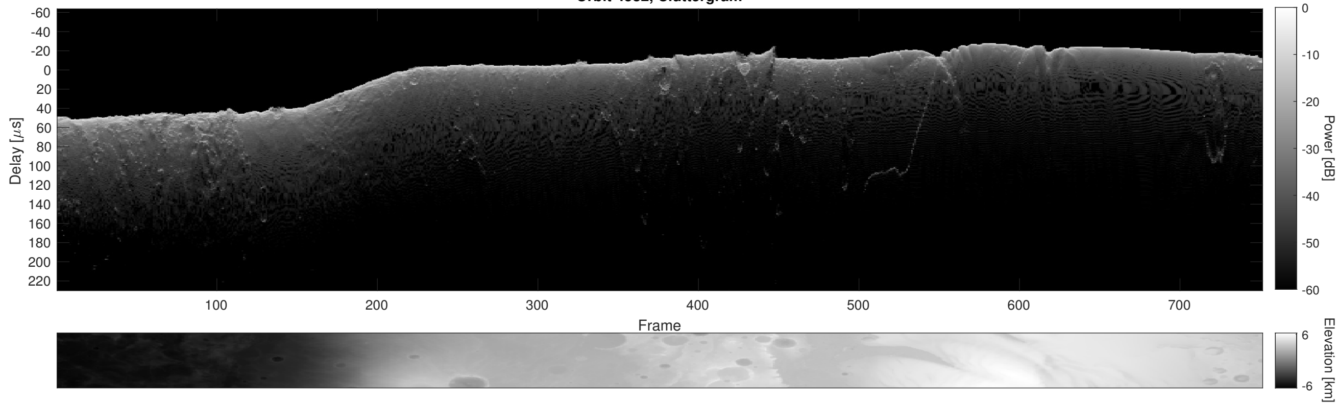
Orbit 4582, Cluttergram
