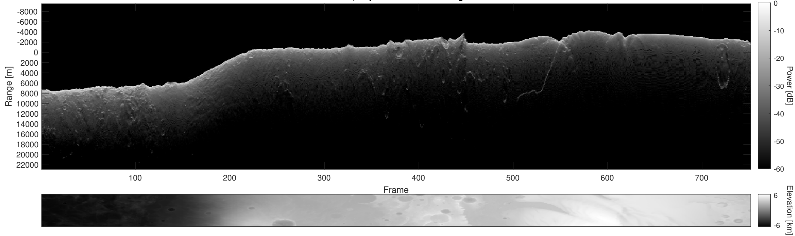
Orbit 4582, Depth-Corrected Cluttergram
