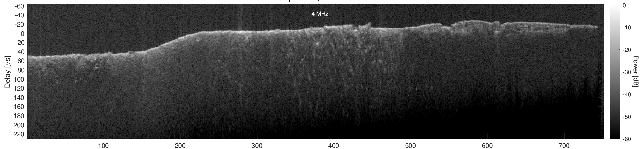
Orbit 4582, Cluttergram
