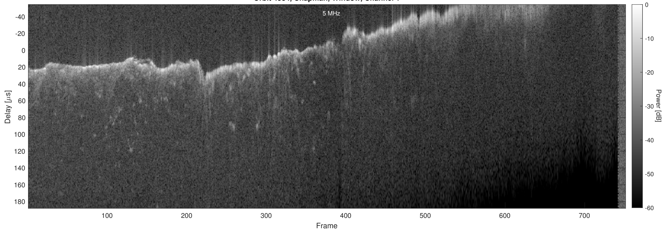
Orbit 4584, Chapman, Window, Channel 2
