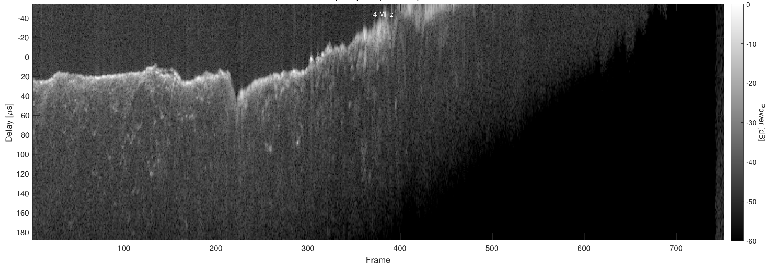
Orbit 4584, Chapman, Window, Channel 2
