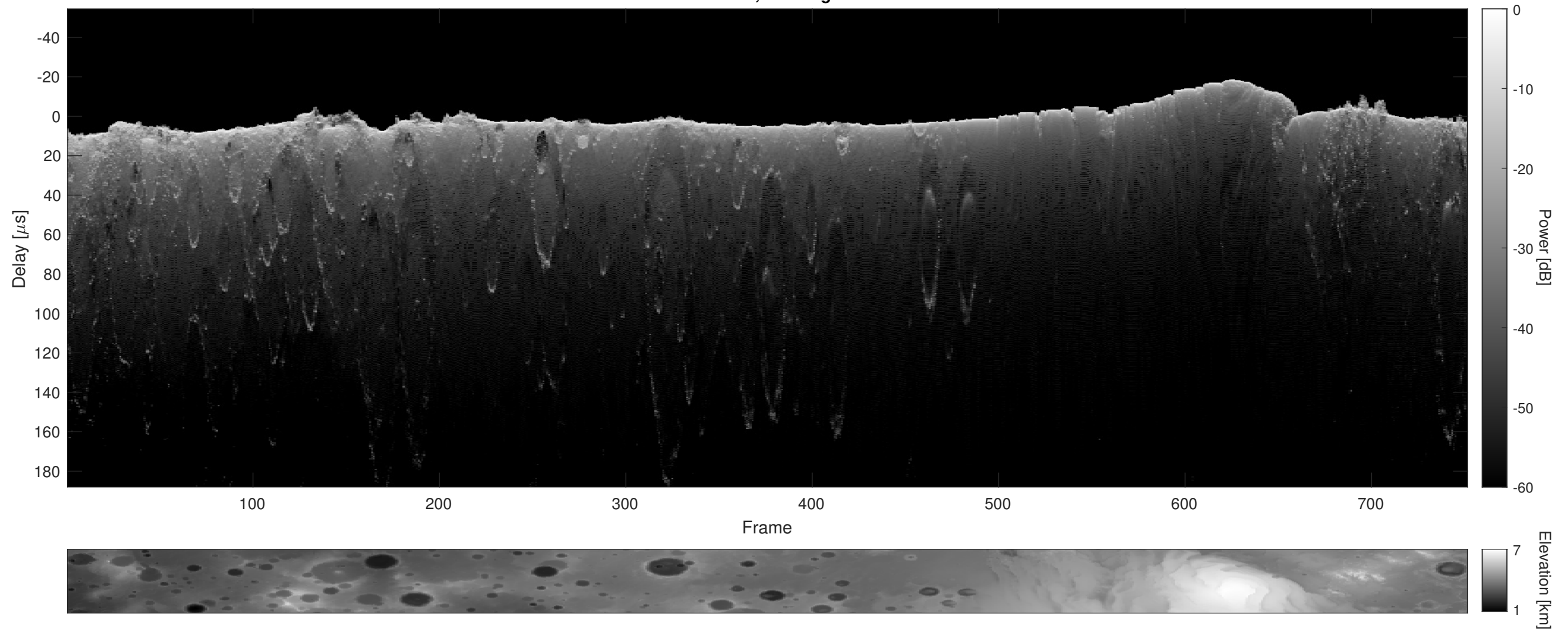
Orbit 4584, Cluttergram
