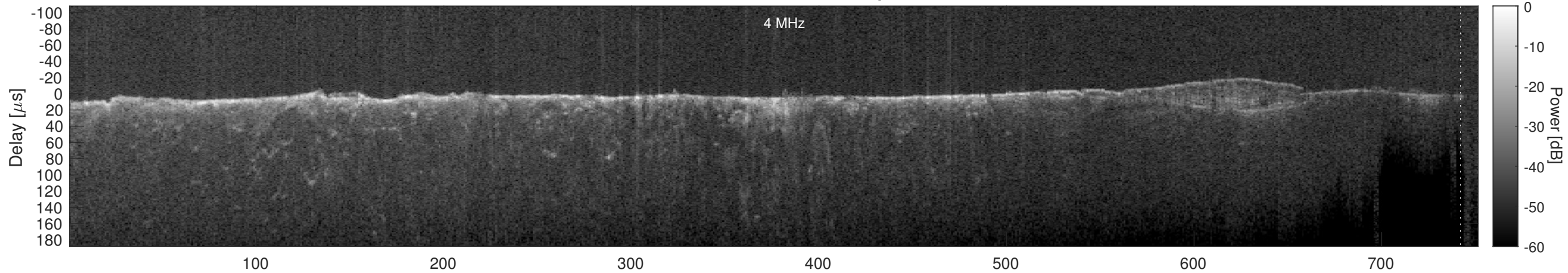
Orbit 4584, Cluttergram
