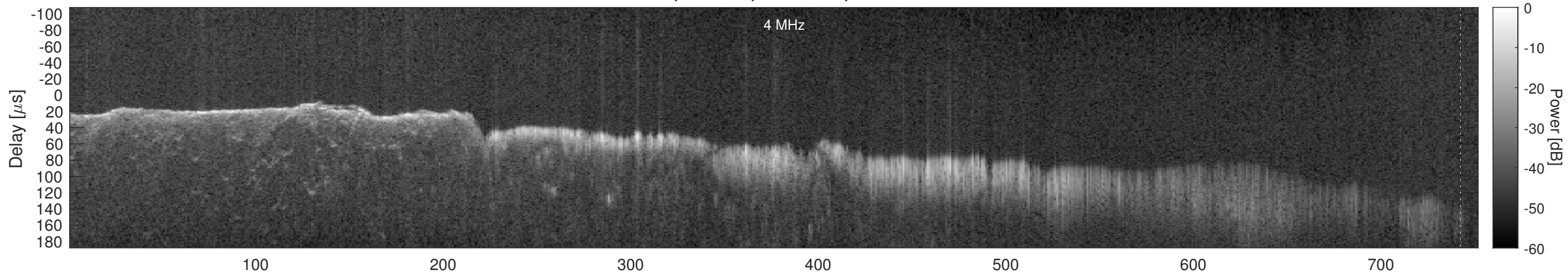
Orbit 4584, Window, Channel 2, Chapman
