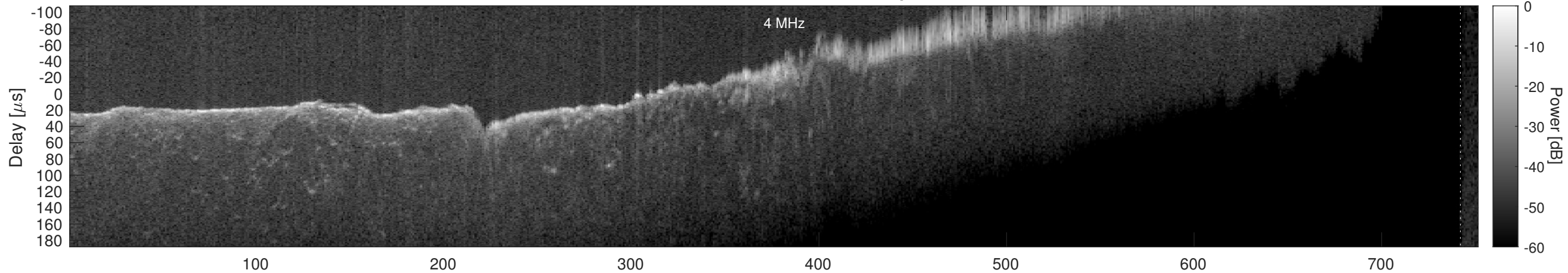
Orbit 4584, Window, Channel 2, Optimized
