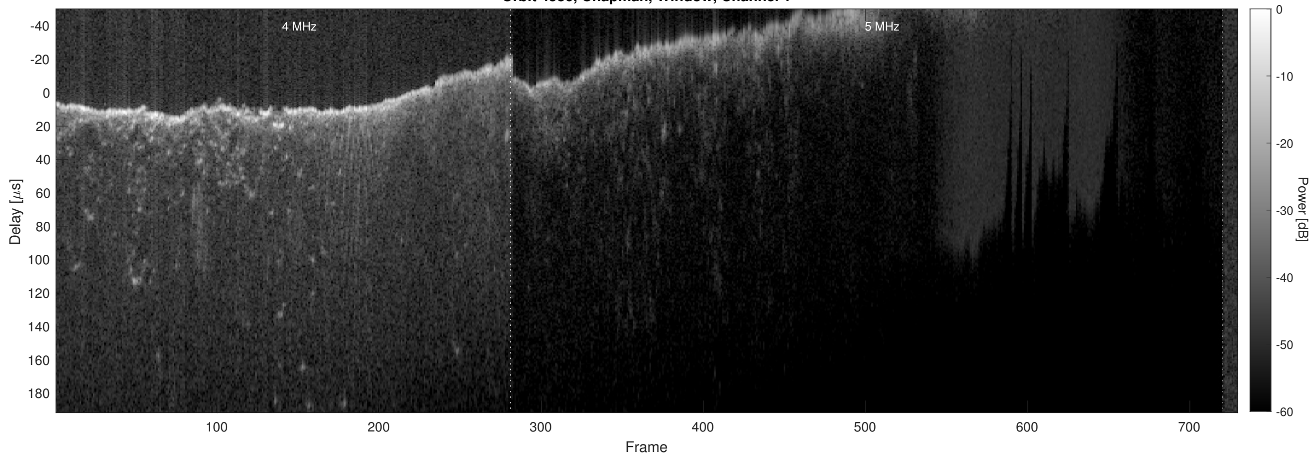
Orbit 4586, Chapman, Window, Channel 2
