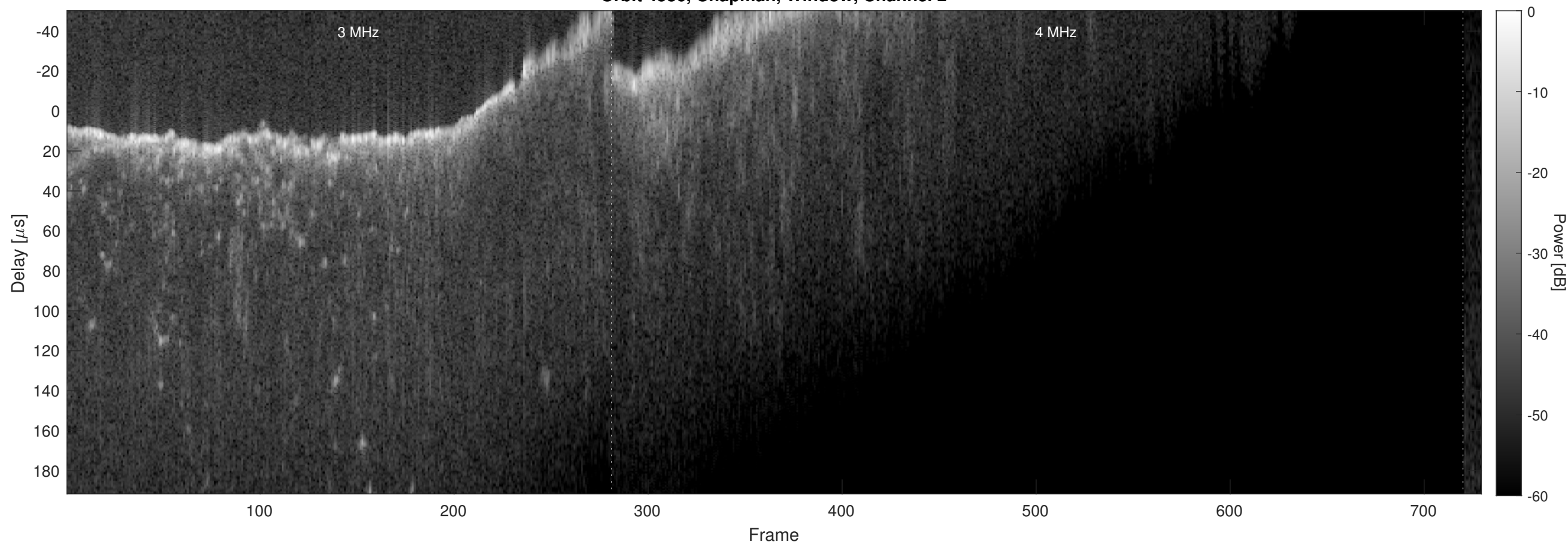
Orbit 4586, Chapman, Window, Channel 2
