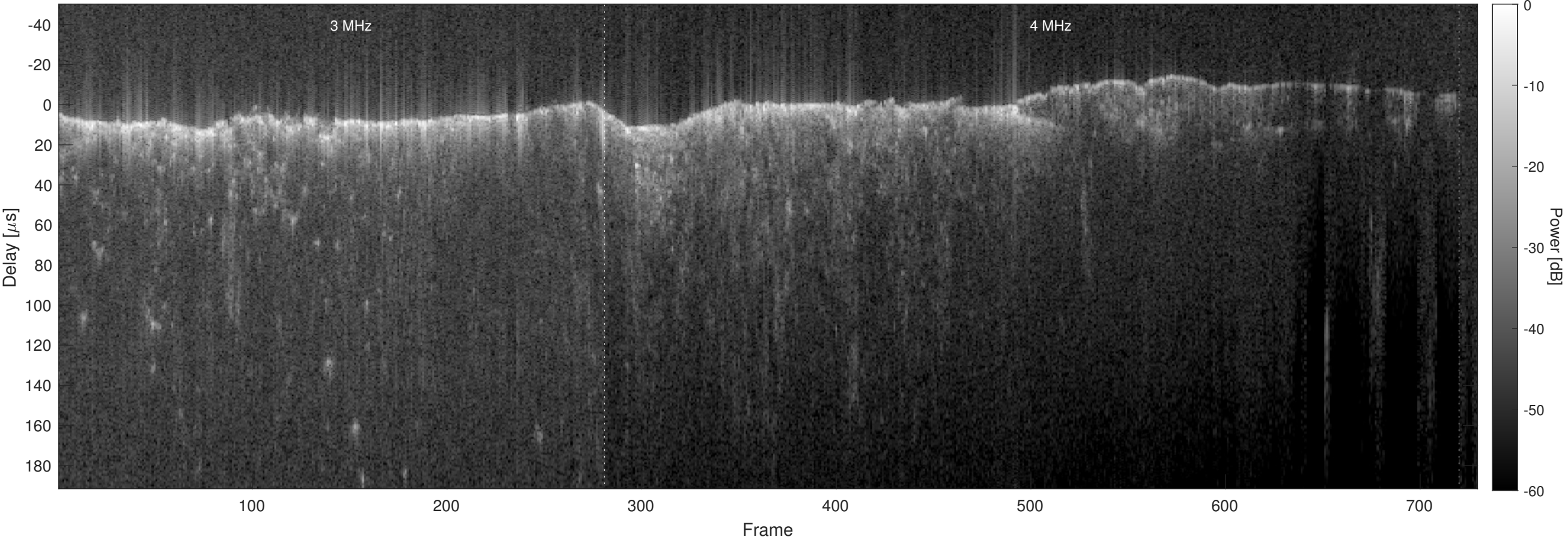
Orbit 4586, Optimized, No Window, Channel 2
