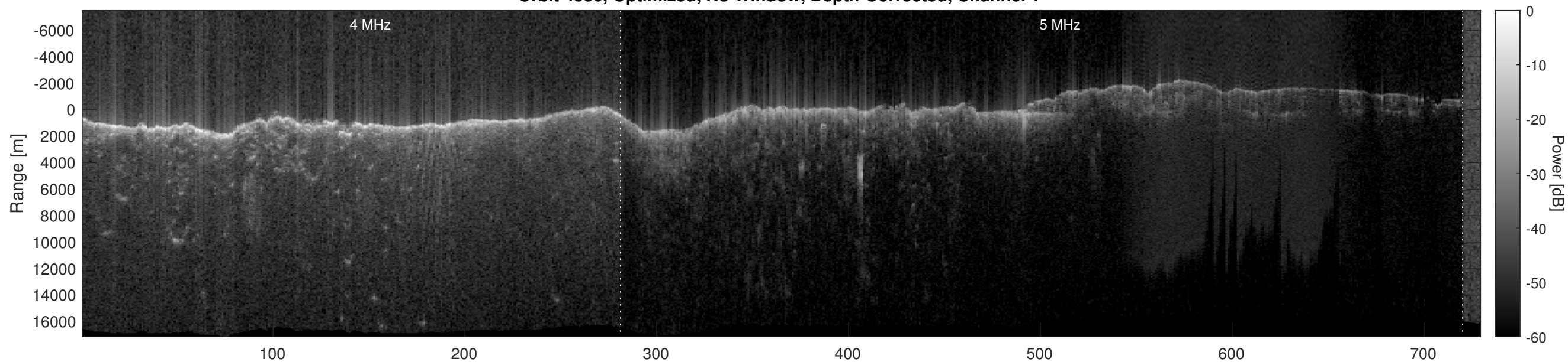
Orbit 4586, Optimized, No Window, Depth-Corrected, Channel 2
