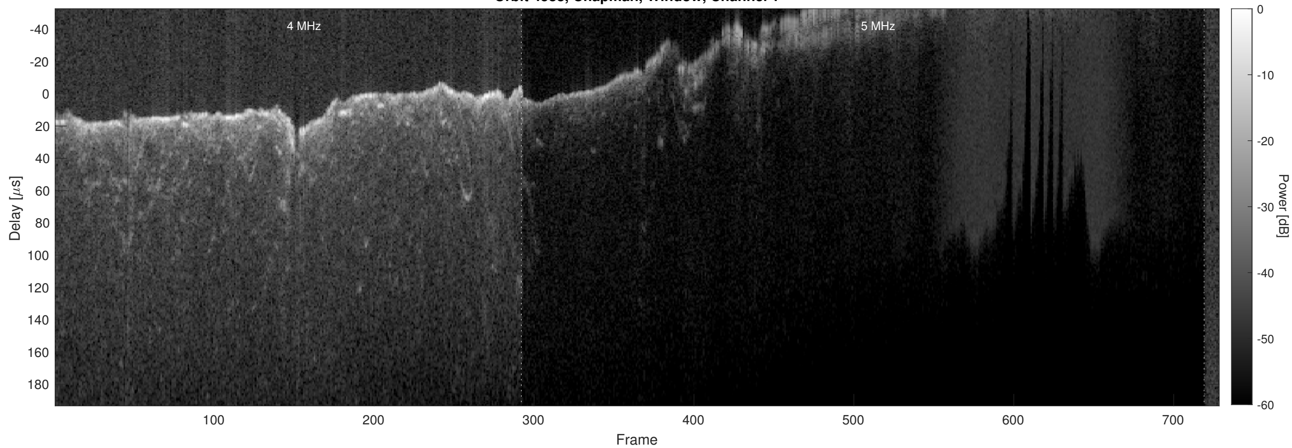
Orbit 4588, Chapman, Window, Channel 2
