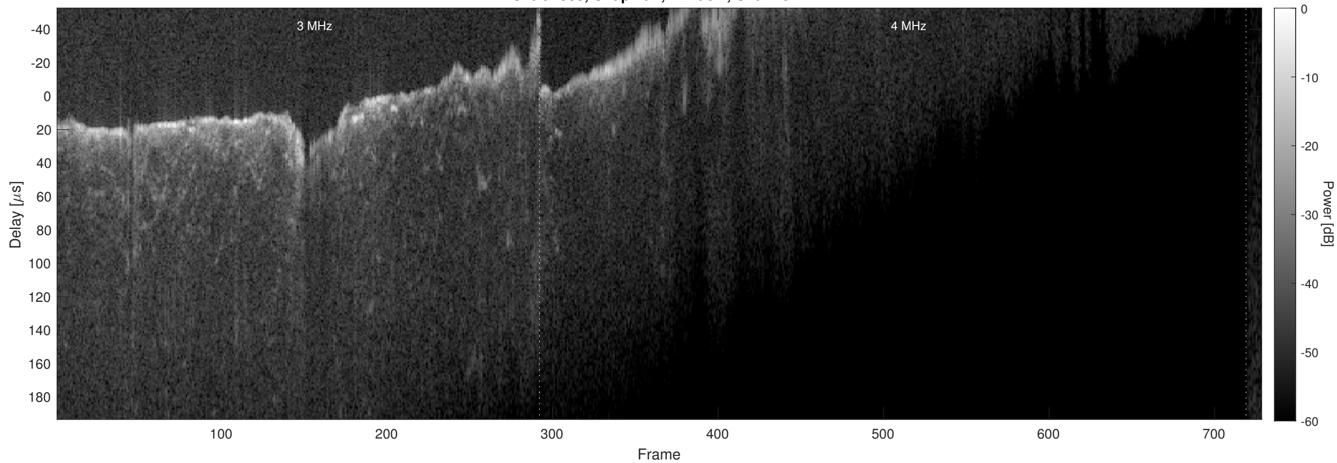
Orbit 4588, Chapman, Window, Channel 2
